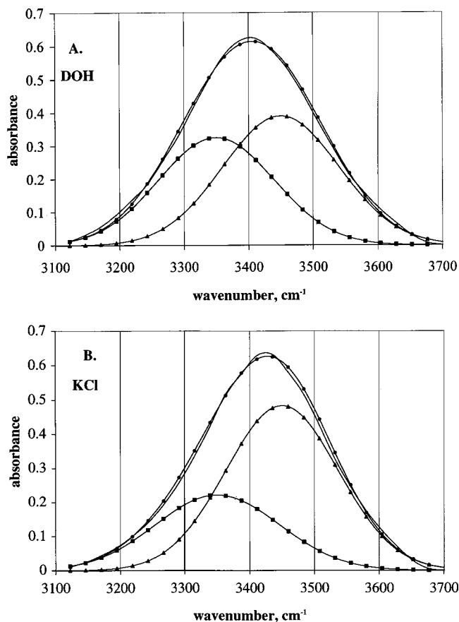
FIG. 2. An example of fits to two Gaussians. Squares represent a Gaussian centered at 3350 cm -1 (width 210 cm -1 ) and triangles are Gaussian centered at 3450 cm -1 (width 212 cm -1 ). Circles are the sum of the two Gaussians and the solid line is the observed experimental curve (from Fig. 1). (A) 5% H 2 O and 95% D 2 O. Respective areas of the fit components: 45% and 55%; (B) 4 molal KCl. Respective areas: 33% and 67%.
